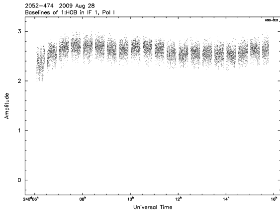
Fig. 3 Amplitude vs time plot for the calibrated 2052-474 observation. Note the downturn in amplitude at the beginning of the experiment. This corresponds to low elevation of the source and is thus likely a residual elevation effect. This is perhaps due to the simple nature of the gain-elevation curve for the Hobart Antenna
