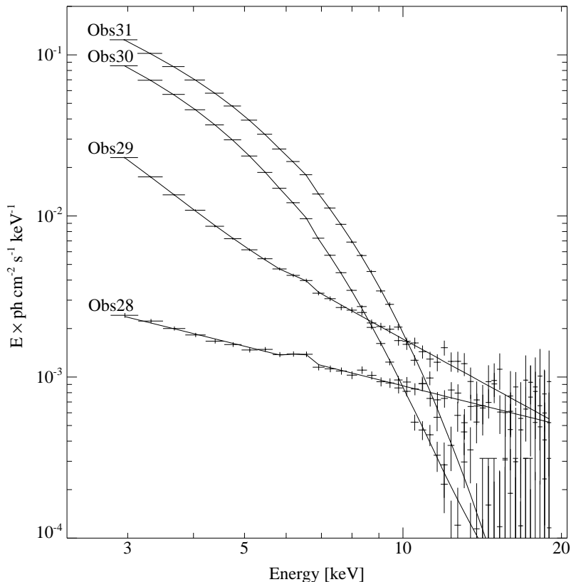
Figure 1.6: Spectrum of LMC X-3, showing a transition from the hard to the soft state. (Wilms et al., 2001, Fig. 4)
