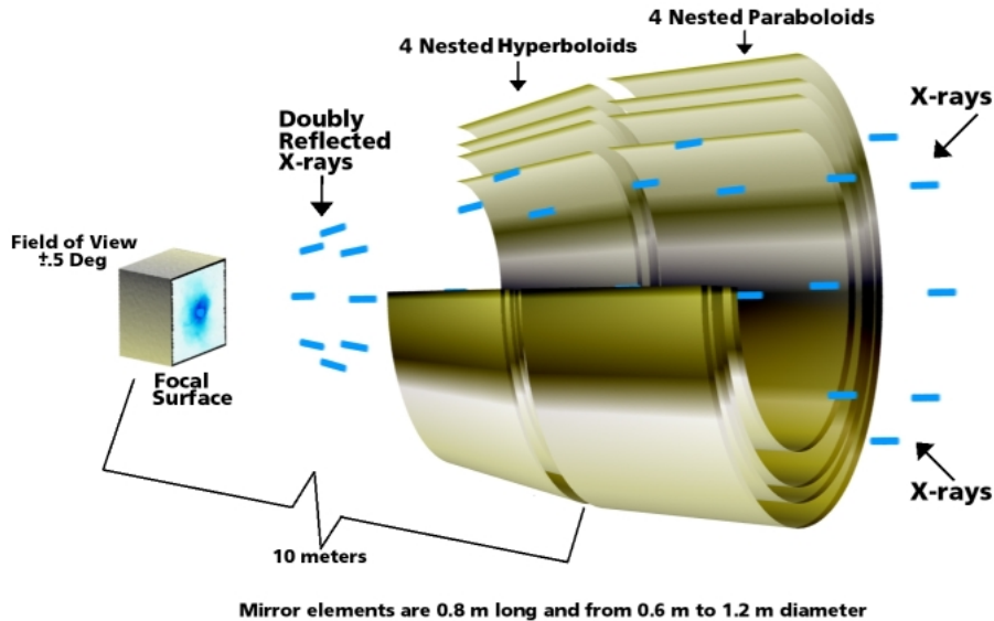
Figure 1.16: Chandra 's high resolution mirror assembly. (from http://chandra.harvard.edu/about/telescope_system.html )
