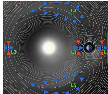
Figure 1.5: The 5 Lagrangian points. (from http://map.gsfc.nasa.gov/m_mm/ob_techorbit1.html )
