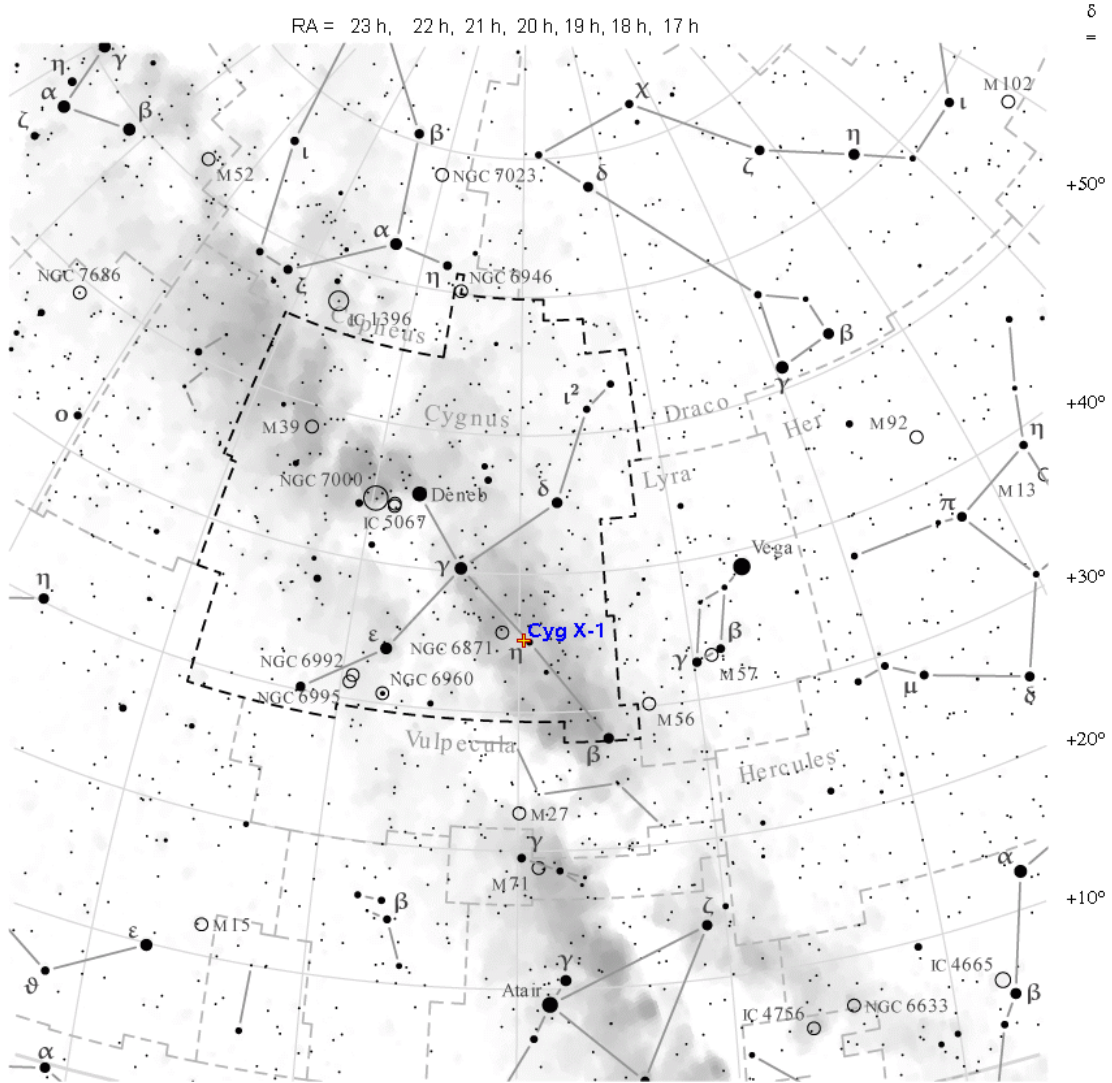
Figure 1.7: The constellation Cygnus with Cyg X-1 at RA = 19^{\text{h}} 58^{\text{min}} 21.7^{\text{s}} , \delta = +35^{\circ} 12' 06'' . (after http://ephemeriden.com/images/charts/cygnus.png )
