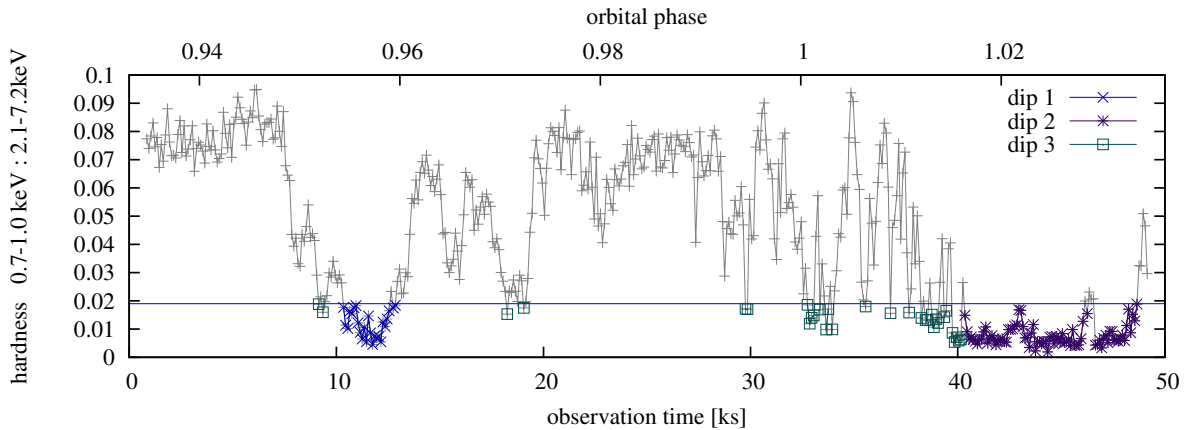
Figure 4.15: Definition of the ‘dip’ sub-spectra (see text).
