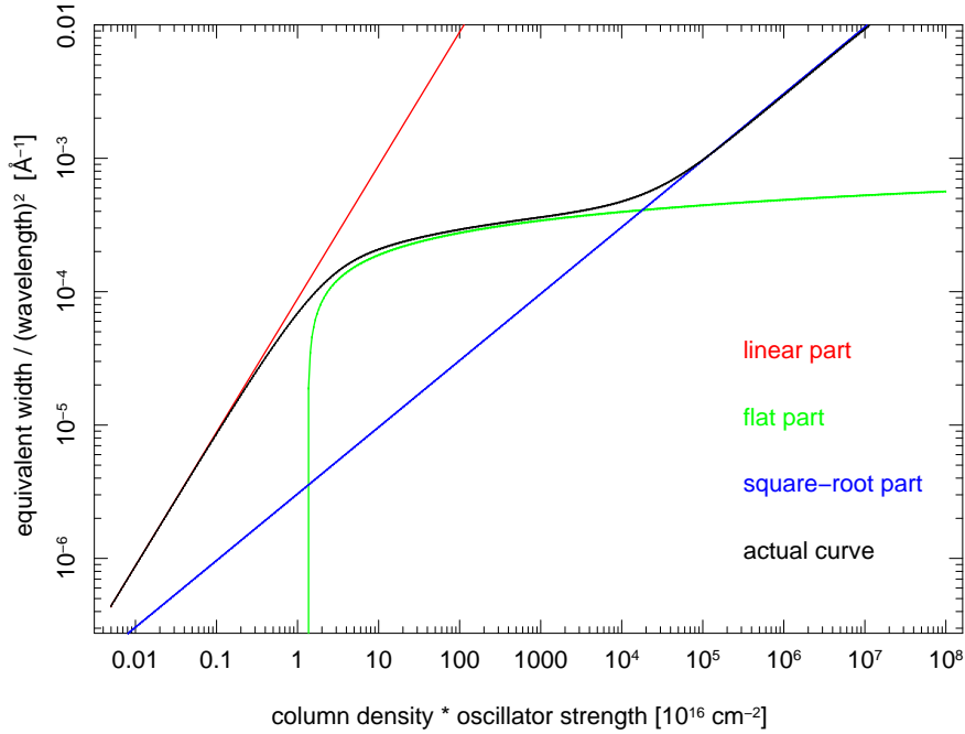
Figure 2.4: A curve of growth in the form W_\lambda/\lambda^2 vs. N_i f_{ij} . In this curve, the linear part is universal and the square-root part only scales with \Gamma . (Here, the parameters \lambda = 5 \text{ \AA} , v_{\text{therm}} = 100 \text{ km s}^{-1} and \Gamma = 10^{12} \text{ s}^{-1} were used.)
