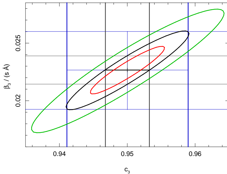
Figure 2.9: \chi^2 contours for single parameter confidence levels.
