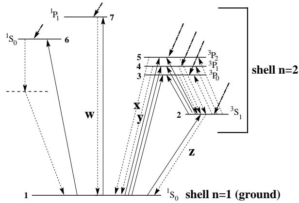
Figure 2.3: A simplified Grotrian diagram of He-like ions. Dashed arrows denote radiative transitions, full arrows show collisional excitations. (Porquet & Dubau, 2000, Fig. 1)
