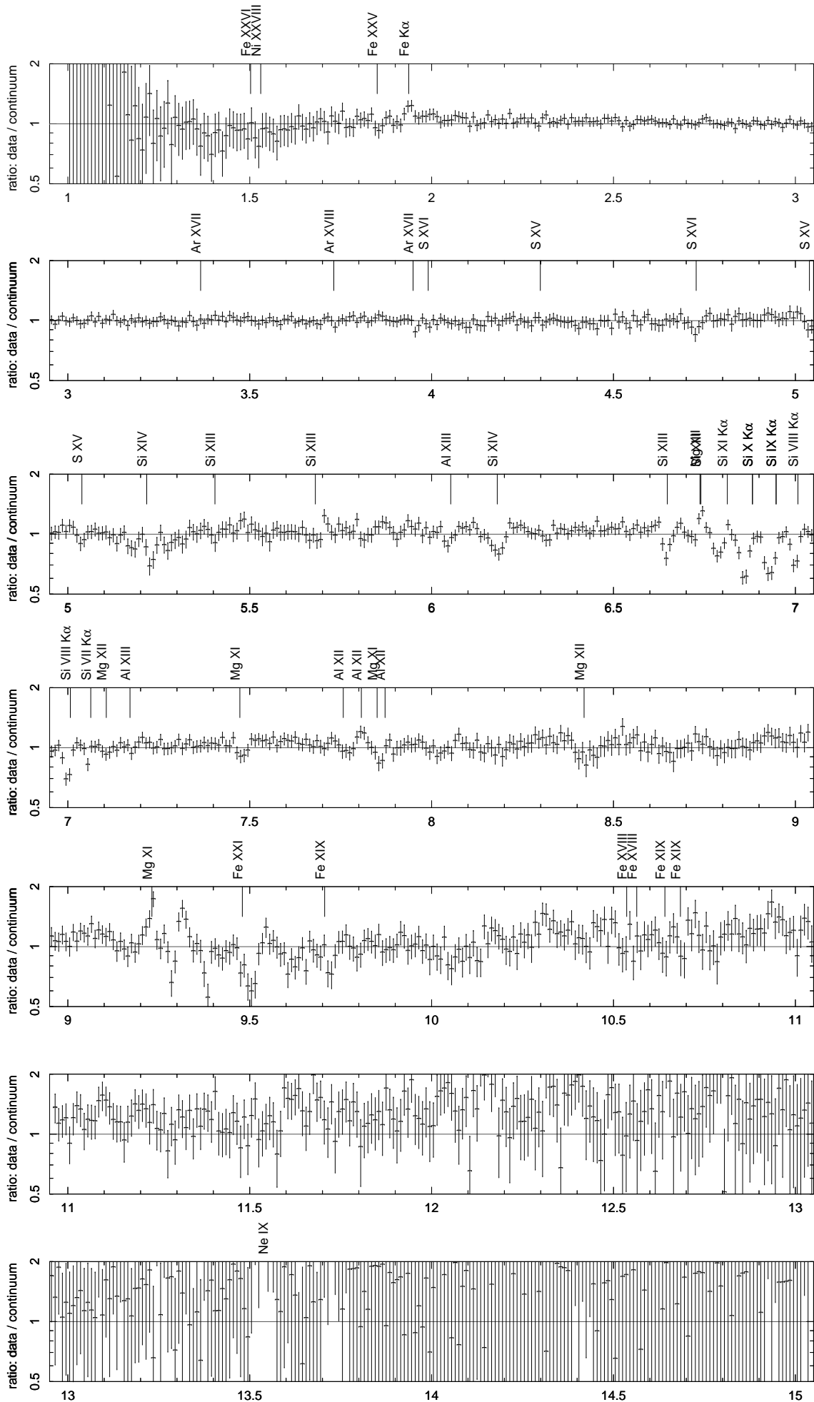
Figure 4.18: Normalized 'dip'-spectrum (data/continuum-ratio) vs. wavelength in Å.
